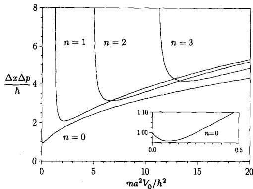
Fig. 1. \Delta x \Delta p / \hbar for several states of the one dimensional square well.
