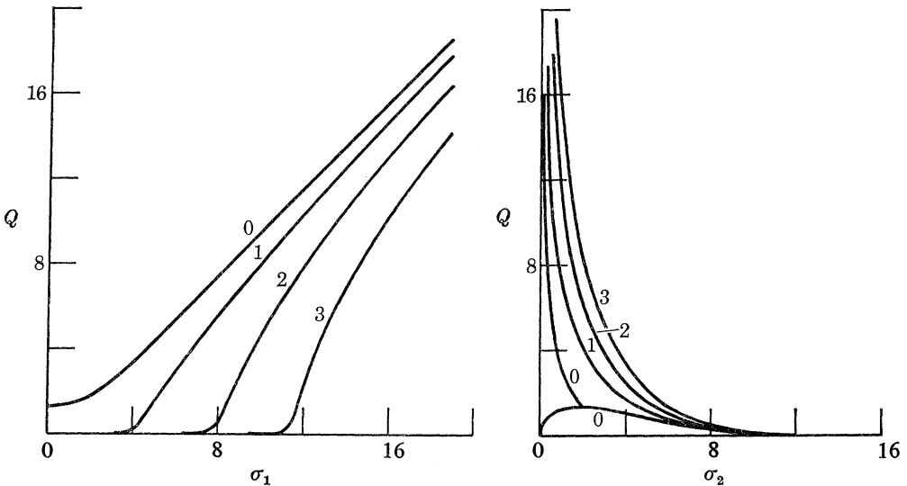
FIGURE 1. The complex frequencies ( \sigma_1 + i\sigma_2 ) belonging to the quasi-normal modes of a rectangular barrier. The frequencies are measured in units of the width of the barrier ( a ); and Q^2 (= a^2U) is a measure of the height of the barrier. The curves are labelled by the values of -n to which they belong.
