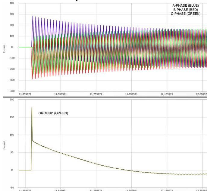
Figure 5 – Initial Asynchronous Energization (Comtrade File)
