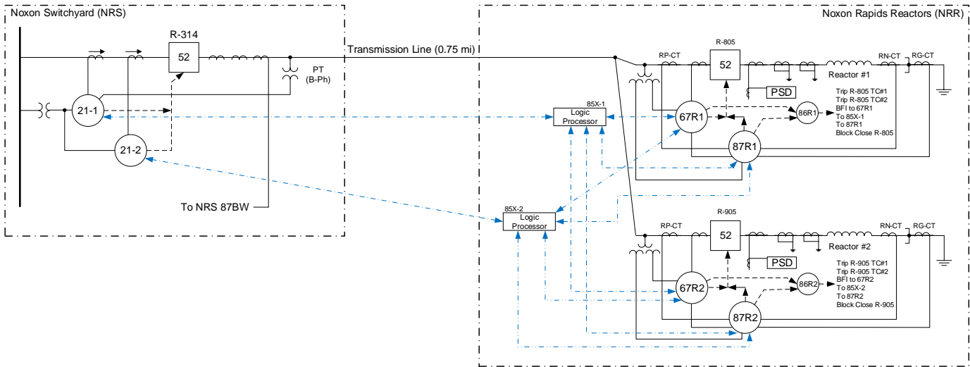
Figure 4 – System Protection Online
