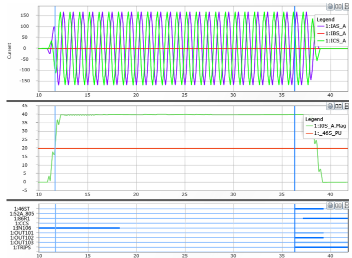
Figure 7 – B-Phase Closure Failure
