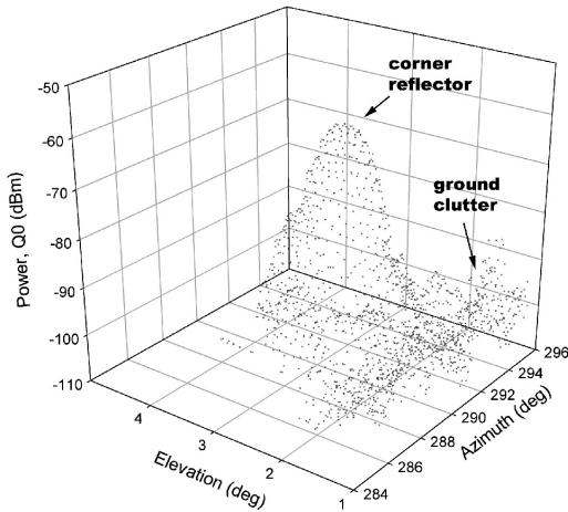
NOAA/D Calibration with Corner Reflector 08JUN99, 2239 UTC, Gate 67 Using NOAA/C Antenna (cfVV-up)
