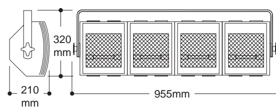
Coda 500W/4
